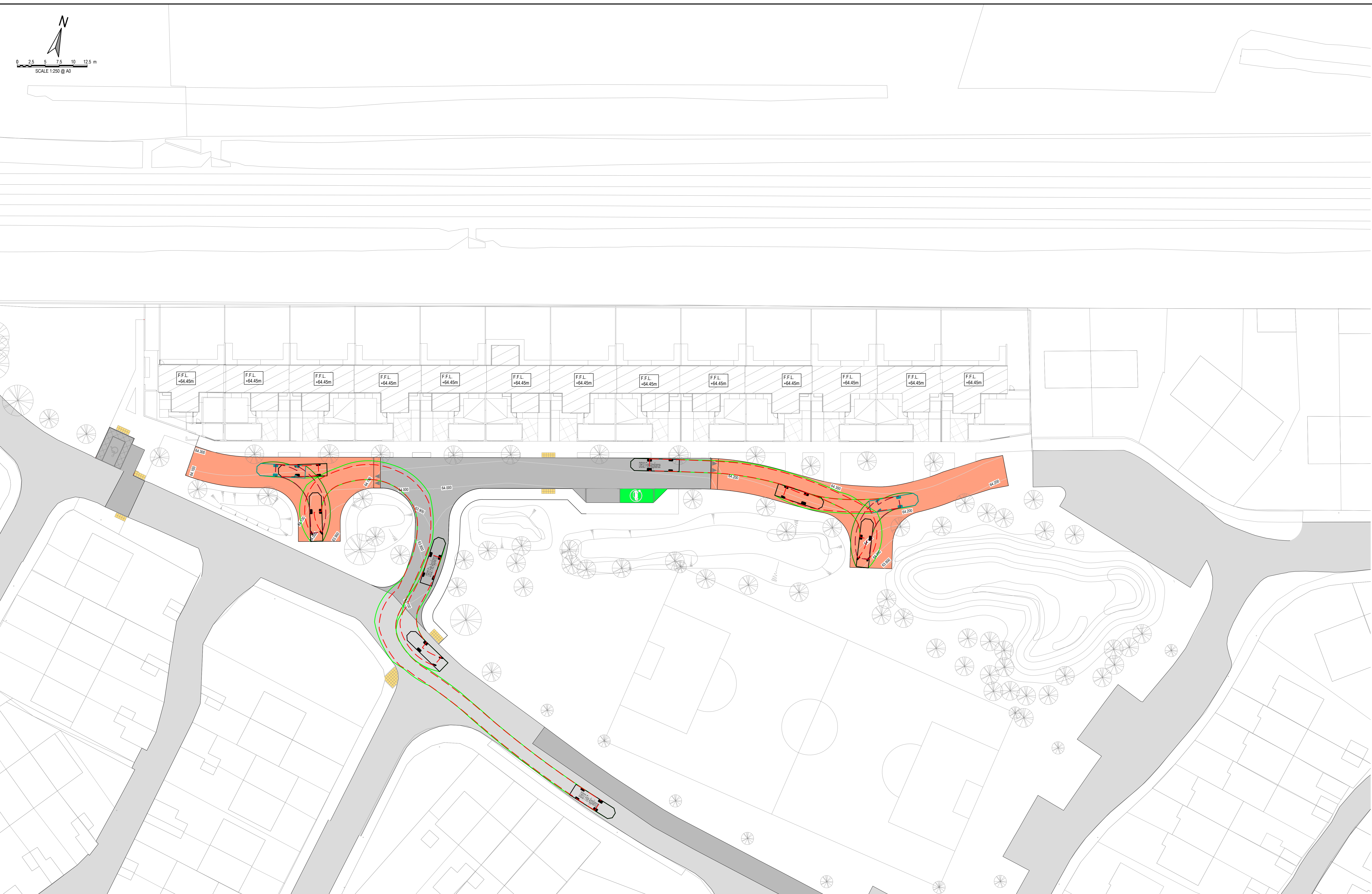
FIRE TENDER SWEPT PATH ANALYSIS SCALE 1:250
