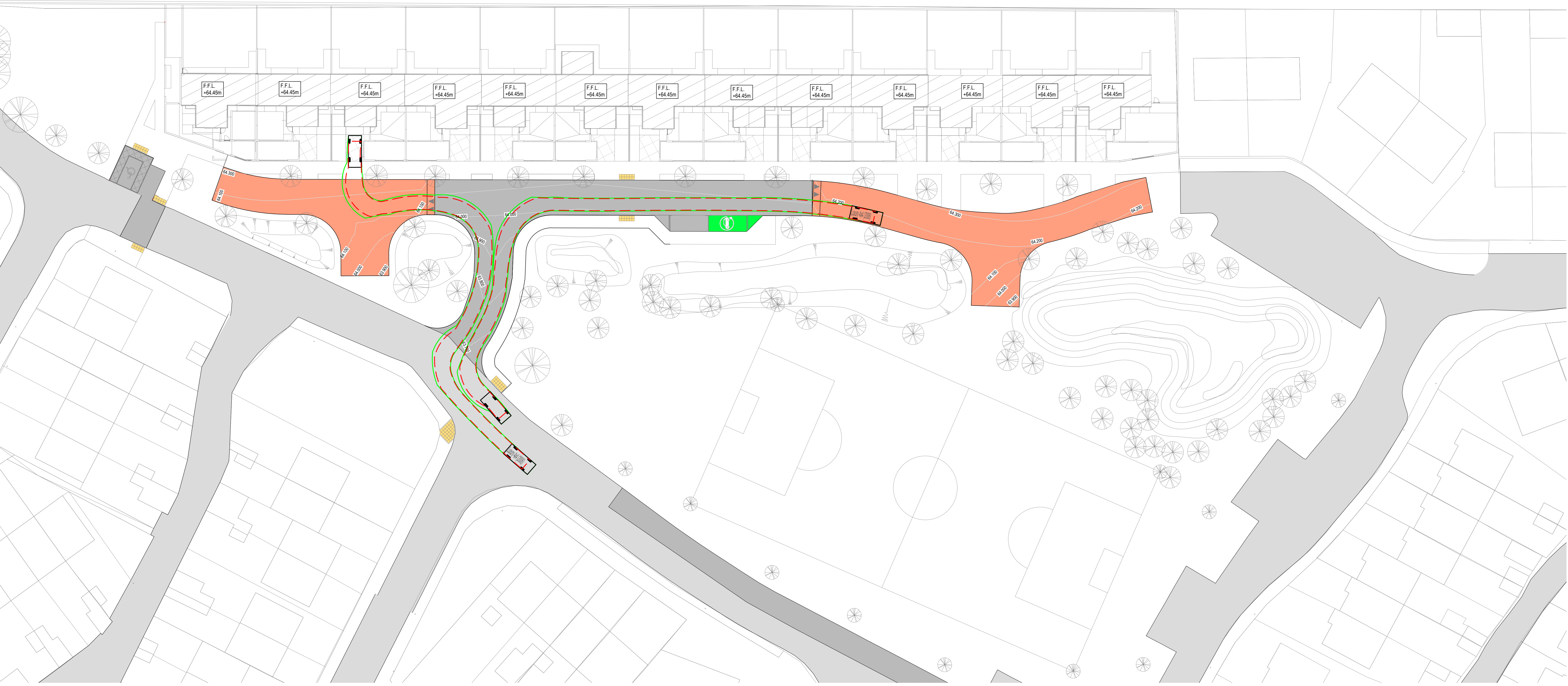
LUXURY 4X4 SWEPT PATH ANALYSIS SCALE 1:250
